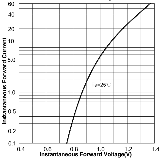
FIG3: Forward Voltage
